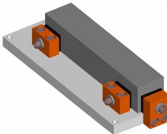
Sample 2 way positioning of a long part
